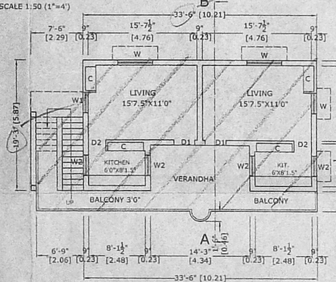
EXG.FIRST FLOOR PLAN
