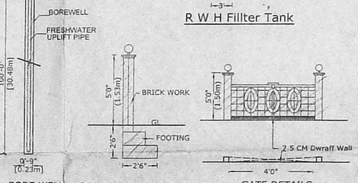
BOREWELL COMPOUND WALL DETAILS SCALE : NTS. GATE DETAILS
