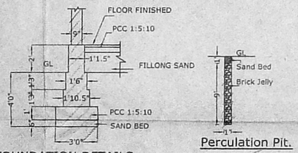
FOUNDATION DETAILS. SCALE 1:50 (1"=4") Percolation Pit.
